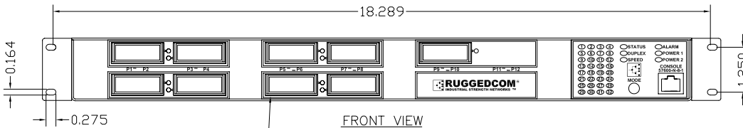
FRONT VIEW
