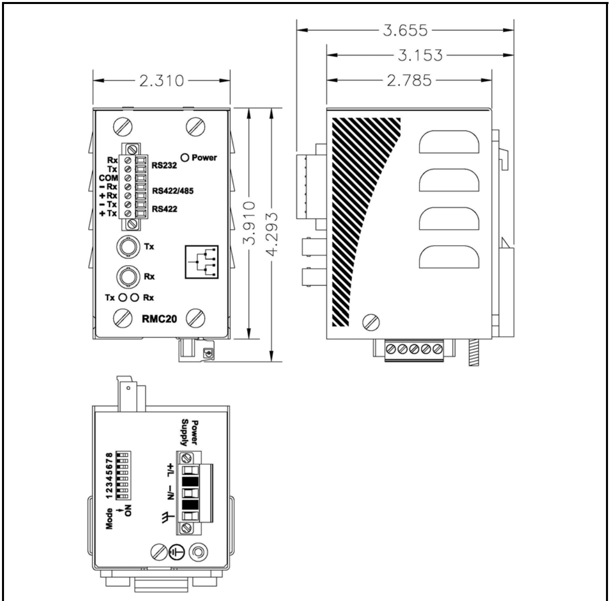
Figure 12: Mechanical Dimensions
